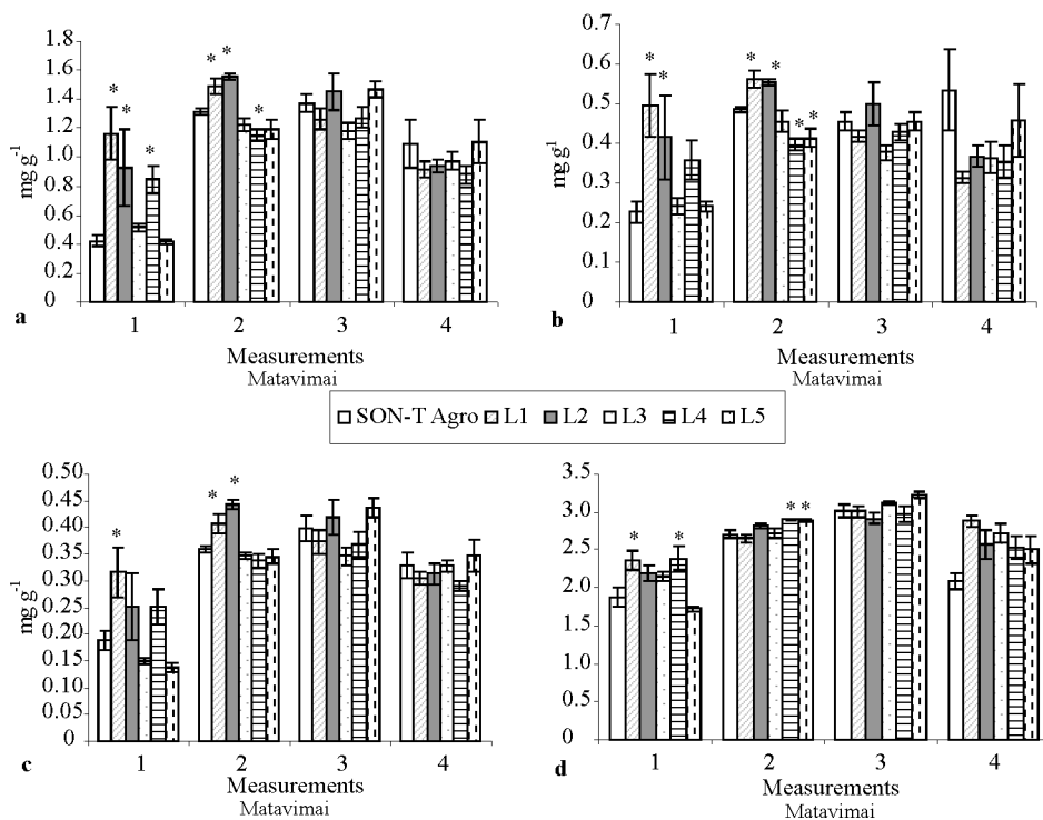
Fig. 1. Changes in photosynthesis pigment content in tomato leaves after transplantation to the greenhouse. Measurements: 1 – during transplantation, 2 – after two weeks, 3 – after four weeks, 4 – after eight weeks in the greenhouse. Significant differences from reference treatment are denoted by an asterisk (*) at p \leq 0.05 (mean \pm SE, n = 3 ).
